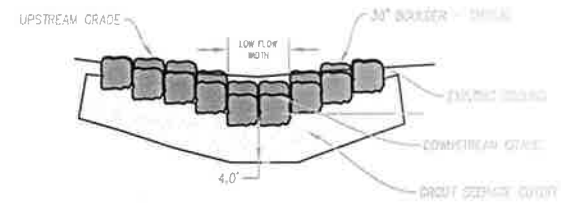
3 UPSTREAM BOULDER DROP SECTION
