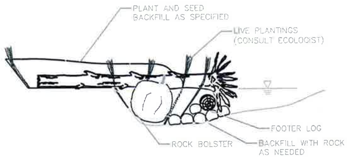
2 ROOTWAD ANCHORED WITH ROCK BOLSTER
