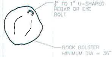
3 ROCK BOLSTER DETAIL
