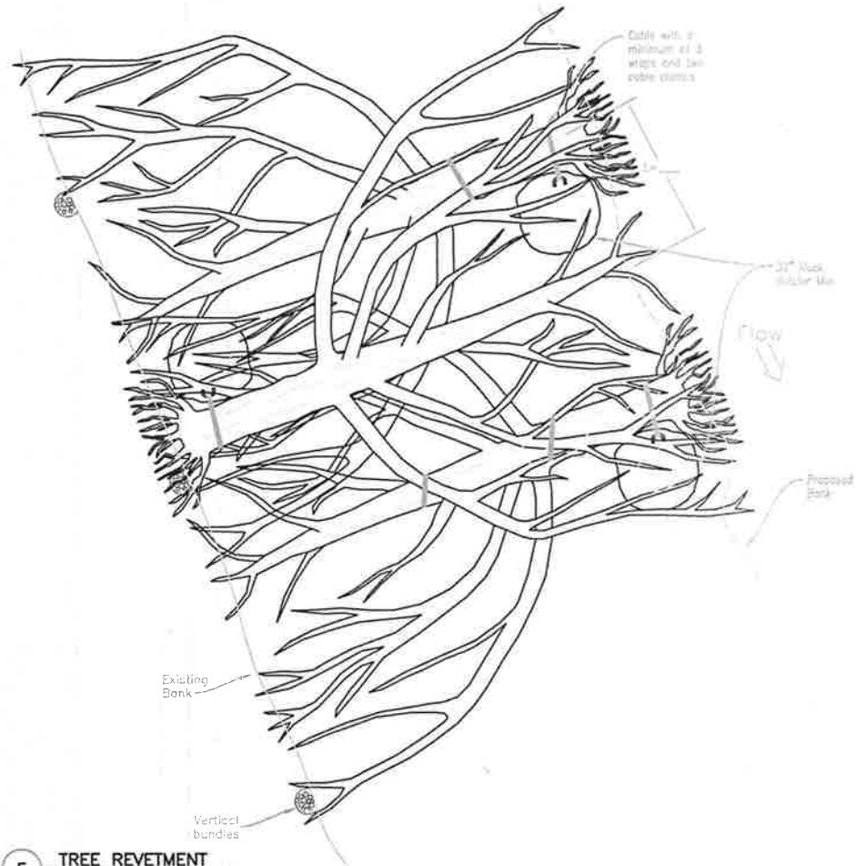
5 TREE REVETMENT
