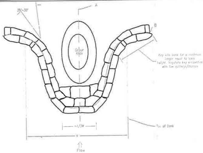
1 ROCK VANE PLAN VIEW
