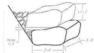
4 TYPICAL ROCK DIMENSIONS AND PLACEMENTS
