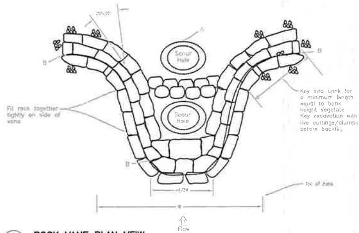
1 ROCK VANE PLAN VIEW
