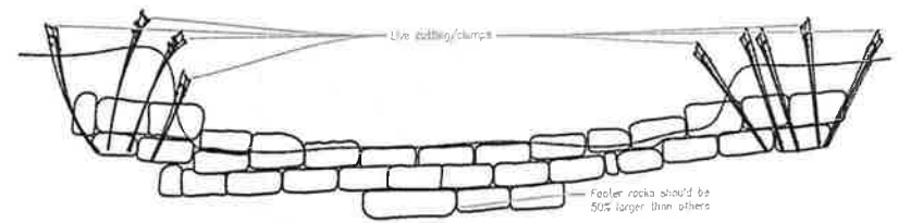
5 ROCK VANE SECTION B
