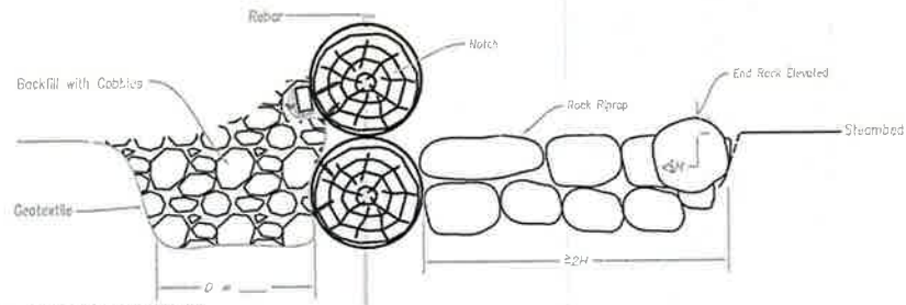
2 CROSS-SECTION
