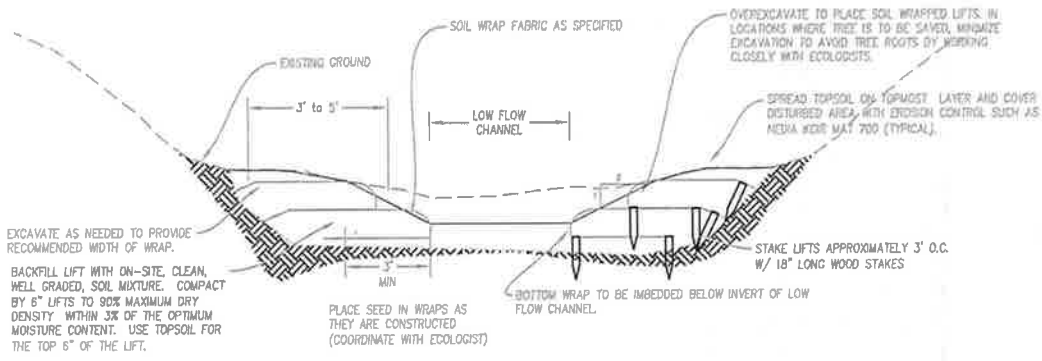
1 SOIL WRAPPED LIFT LOW FLOW CHANNEL EXAMPLE
