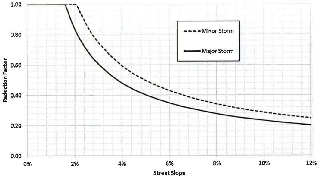
Figure 900-2. Reduction Factor for Gutter Flow (UDFCD, 2016).
