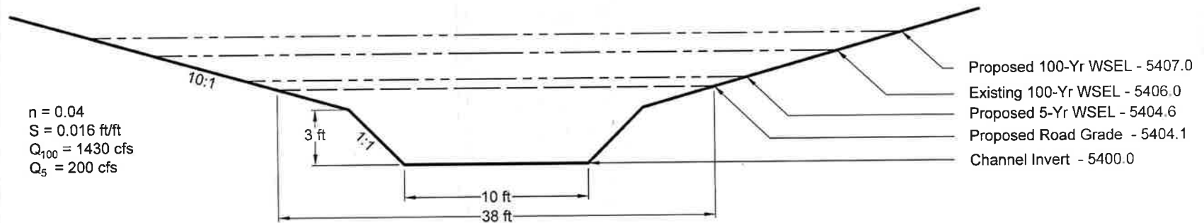
Channel Geometry (Not to Scale)
