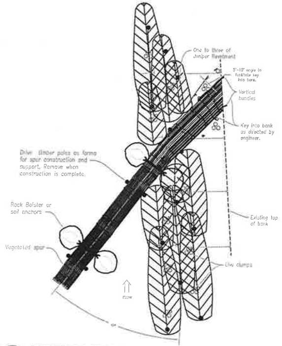
1 VEGETATIVE SPUR WITH JUNIPER REVETMENT
