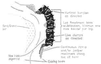
1 TREE REVETMENT FULL LAYOUT
