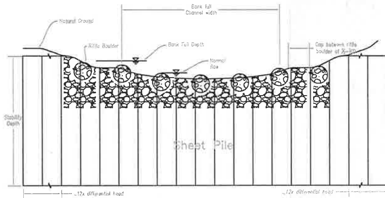
1 CHUTE SECTION VIEW
