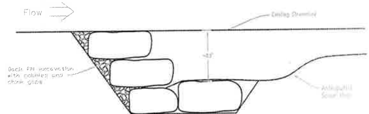
3 ROCK BOLSTER DETAIL
