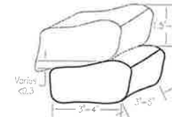
3 TYPICAL ROCK DIMENSIONS AND PLACEMENTS
