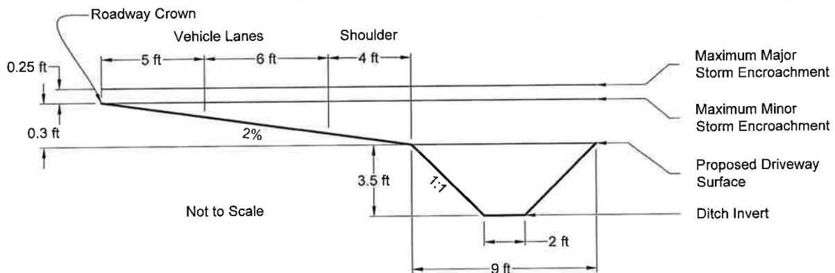
Figure 1000-12. Private Driveway Culvert Example Ditch Geometry.
