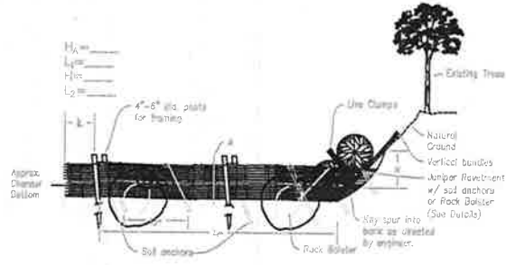
3 VEGETATED SPUR
