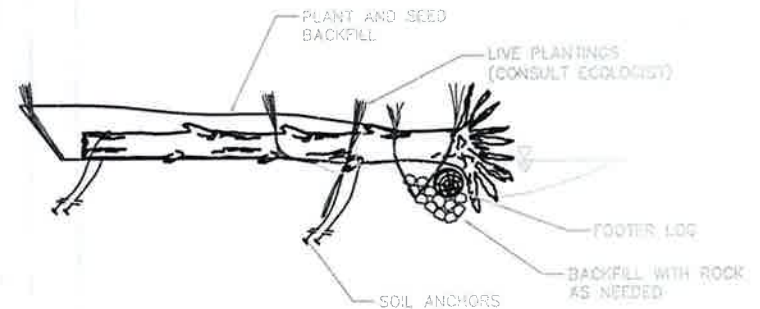
5 ROOTWAD ANCHORED WITH SOIL ANCHORS
