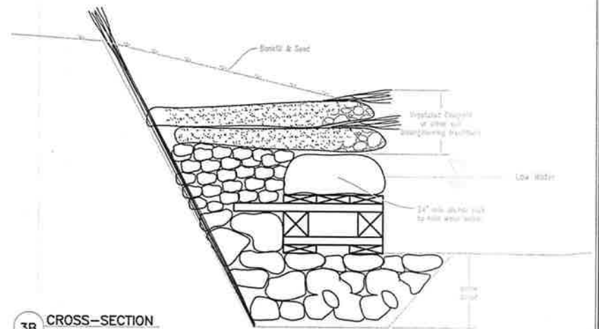
3B CROSS-SECTION
