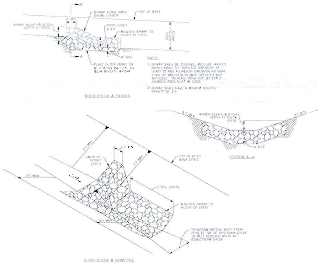
Figure 1100-1. Schematic Roadside Ditch Check Structure.
