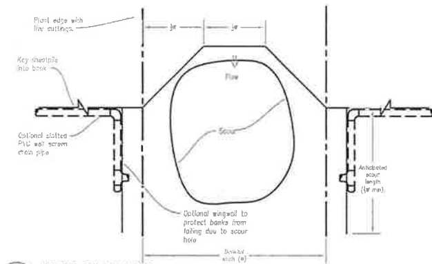
3 WEIR PLAN VIEW
