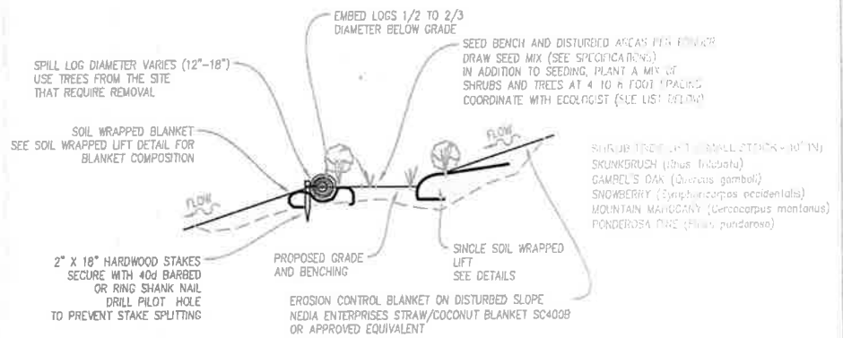
4 LOG GRADE BANK STABILIZATION- EXAMPLE
