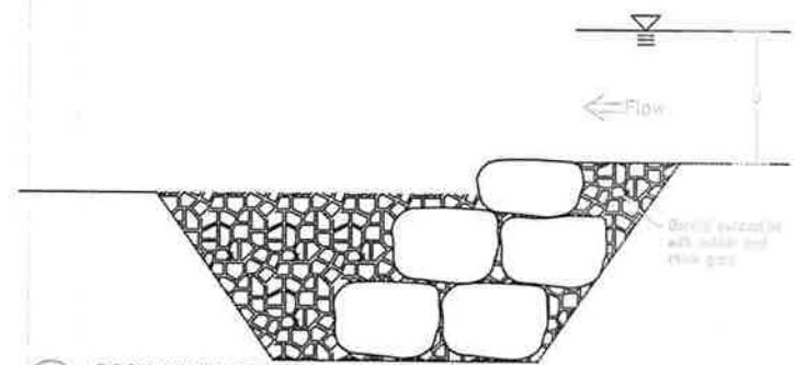
2 ROCK VANE SECTION A
