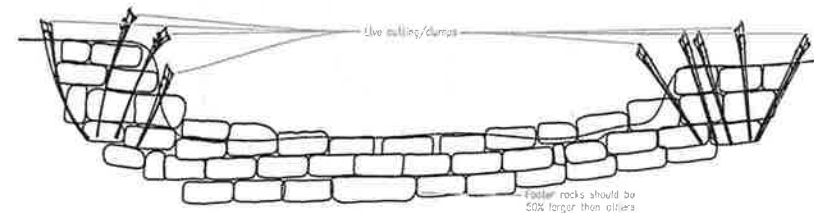
2 ROCK VANE SECTION B
