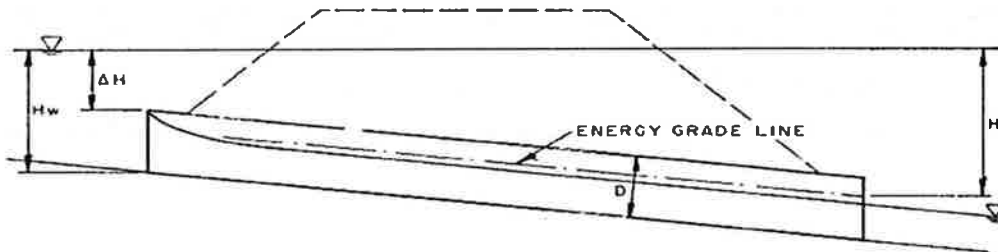
Figure 1000-6. Inlet Control – Submerged Inlet (UDFCD, 2016).
