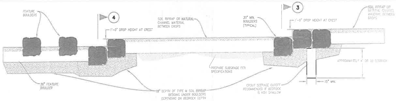
2 CHECK STRUCTURE DROP EXAMPLE - PROFILE
