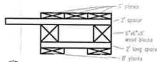
2B SIDE
