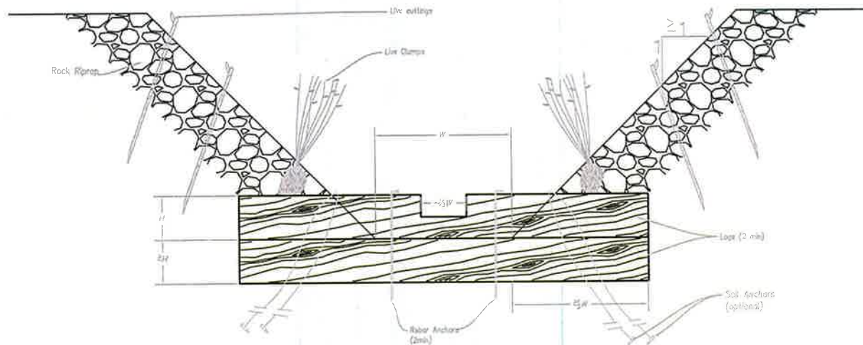
1 FRONT VIEW OF LOG CHECK
