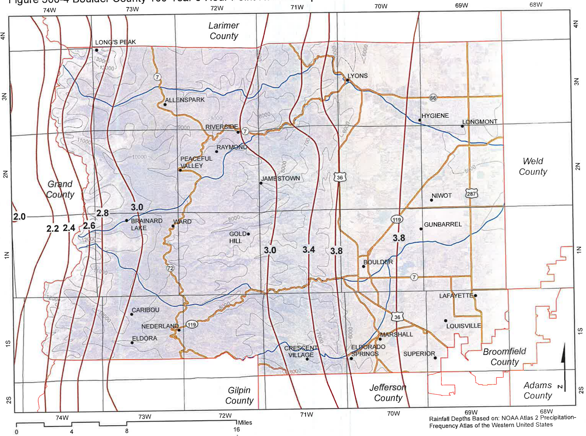
Figure 500-4 Boulder County 100-Year 6-Hour Point Rainfall Depths
