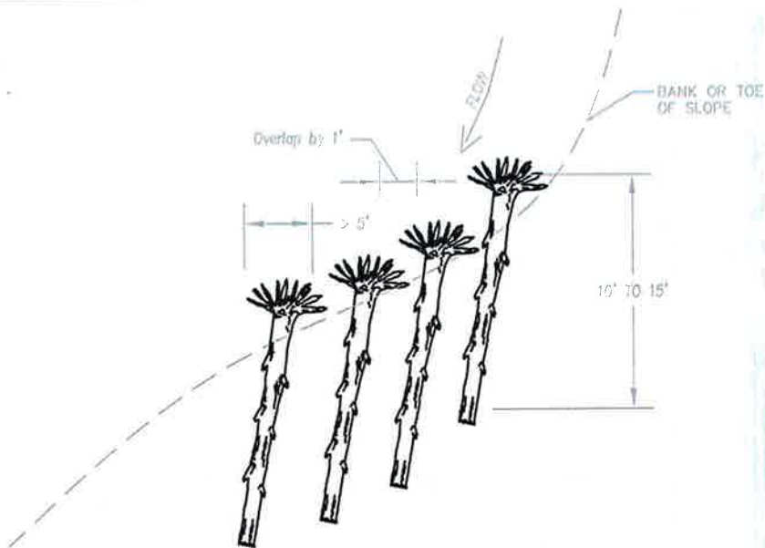
1 ROOTWAD PLACEMENT EXAMPLE PLAN VIEW
