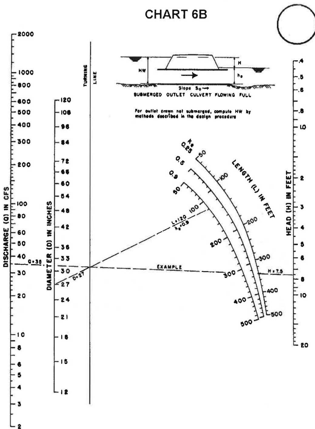
Figure 1000-7 Common Nomographs
