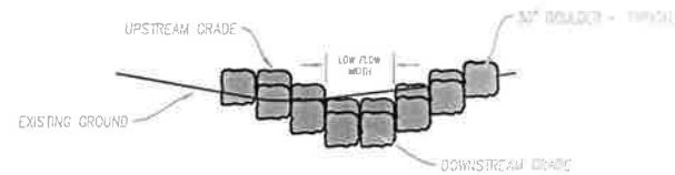
4 DOWNSTREAM BOULDER DROP SECTION
