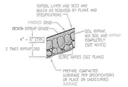
2 SOIL RIPRAP WITH MULCH EXAMPLE
