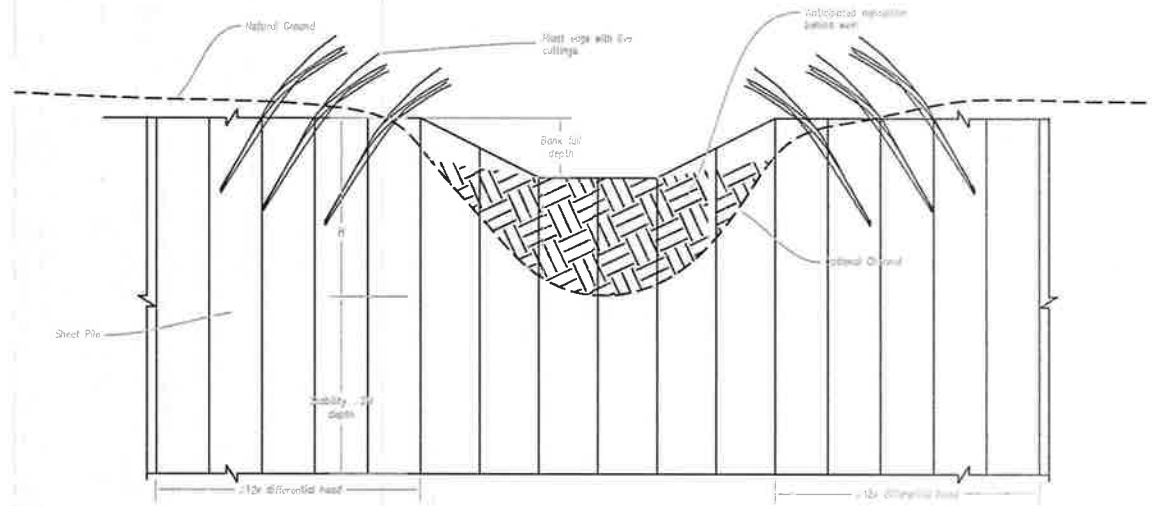
4 WEIR SECTION VIEW
