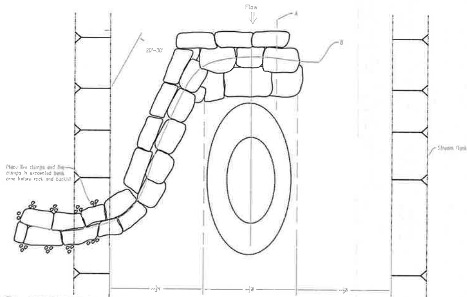
1 HOOK VANE PLAN VIEW
