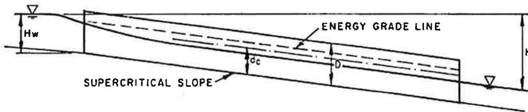
Figure 1000-5. Inlet Control – Unsubmerged Inlet (UDFCD, 2016).
