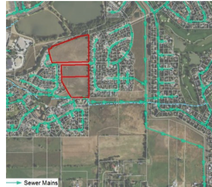
Existing Sewer Mains Source: Wastewater Utility Master Plan, 2009
