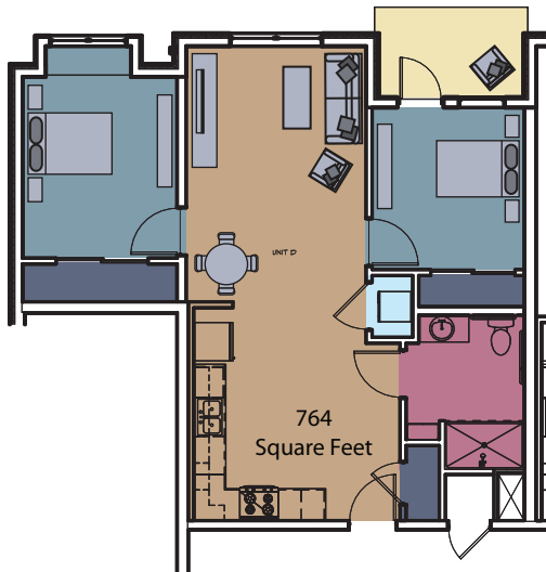
4 UNIT TYPE D FINISH PLAN 1/4" = 1'-0"
