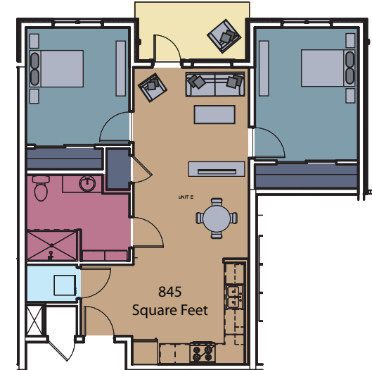
5 UNIT TYPE E FINISH PLAN 1/4" = 1'-0"
