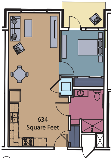
1 UNIT TYPE A FINISH PLAN 1/4" = 1'-0"
