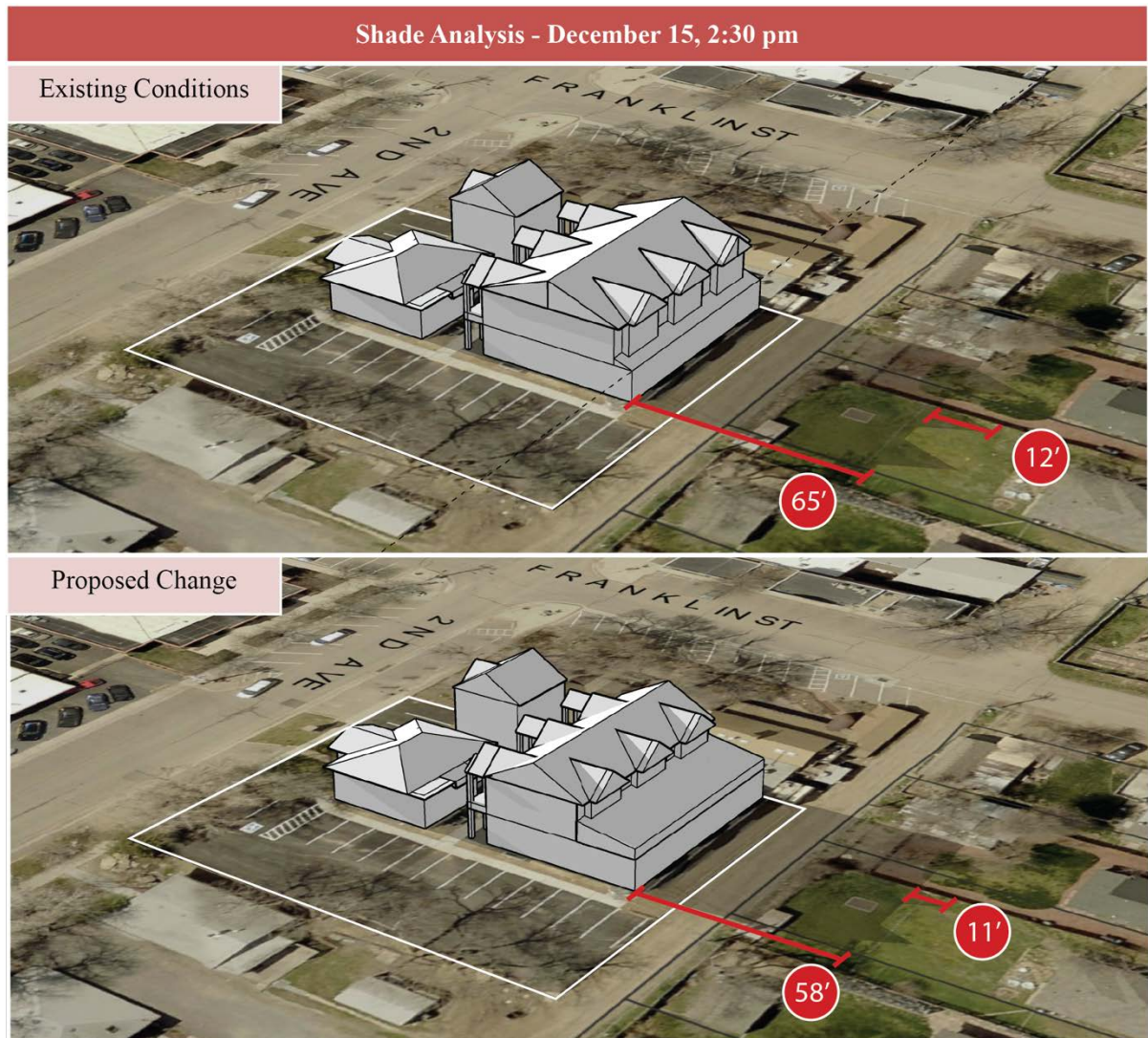
Figure 4. Shade analysis on December 15, at 2:30 pm
