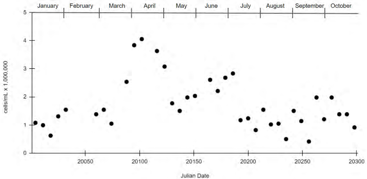
Figure 3: Cyanobacterial cell concentrations in Lagerman Reservoir in 2020 as measured by remote sensing of algal pigments (EPA CyAN).
