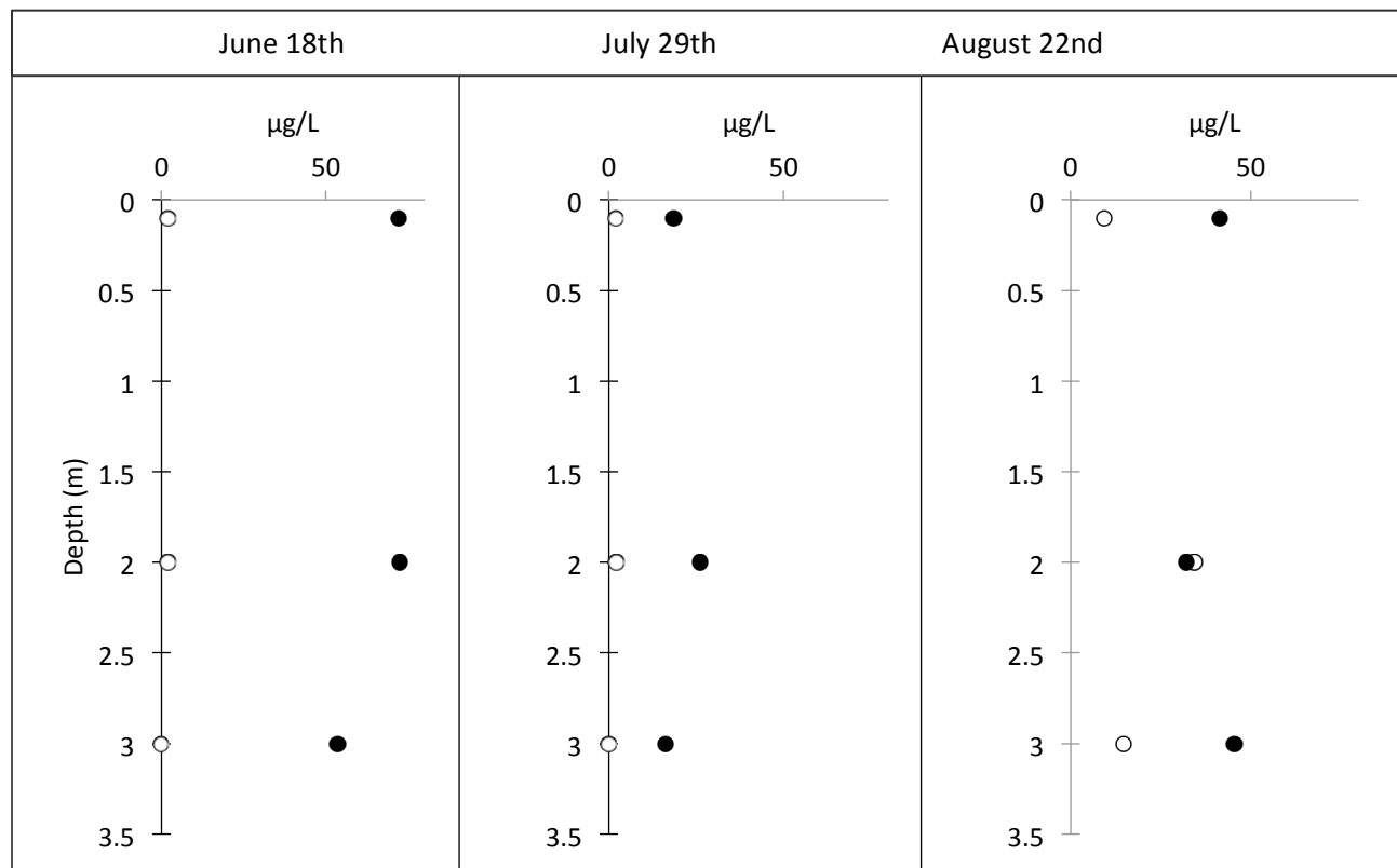
Figure 1: Chlorophyll-a (filled circles) and phaeophytin (hollow circles) concentrations from the water column in Lagerman Reservoir on sampling dates in 2020.
