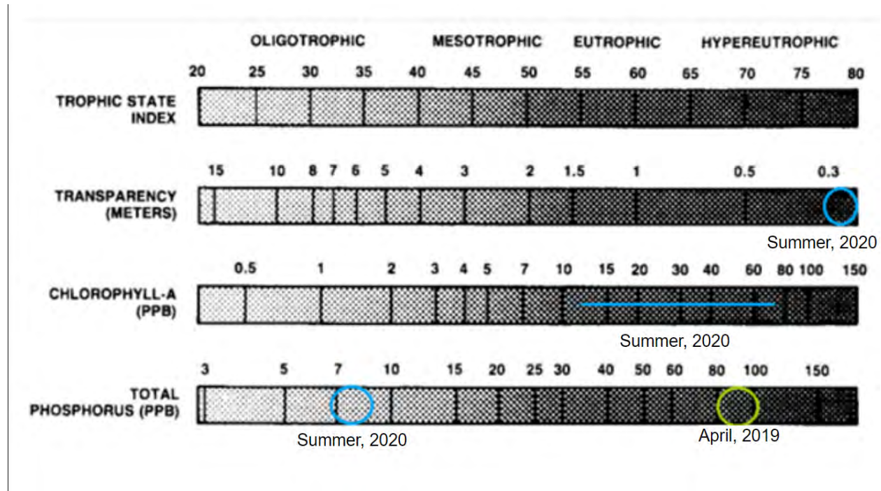
Figure 7: Values for trophic state, transparency, chlorophyll-a, and total phosphorus for Lagerman Reservoir placed on Carlson’s Trophic State Index (Stednick 2003).
