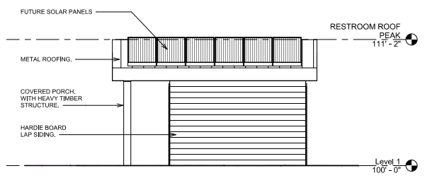
Vault Restroom South Elevation 1/4" = 1'-0"
