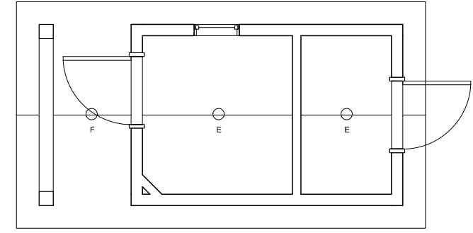
Vault Restroom Ceiling Plan 1/2" = 1'-0"
