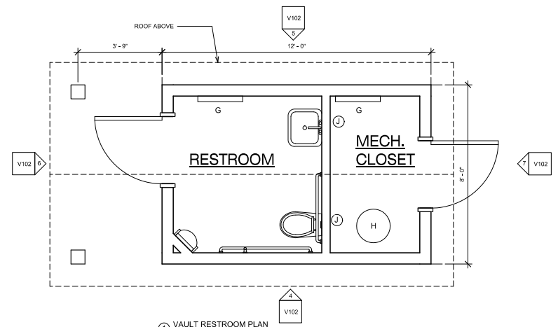
Vault Restroom Plan 1/2" = 1'-0"
