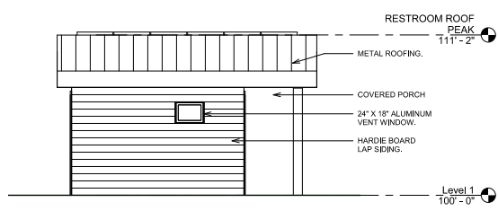
Vault Restroom North Elevation 1/4" = 1'-0"
