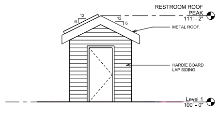
Vault Restroom East Elevation 1/4" = 1'-0"
