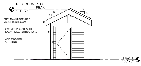
Vault Restroom West Elevation 1/4" = 1'-0"
