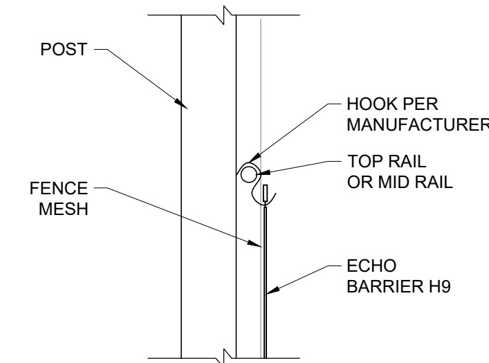
1 ECHO BARRIER CONNECTION DETAIL 4 SCALE: NTS
